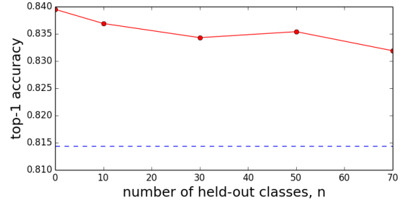
Figure 6. Image classification on Food-101N in terms of top-1 accuracy (%). Red line shows the results when verification labels in n/101 classes are held out for CleanNet. The blue dashed line shows the baseline without using CleanNet.
