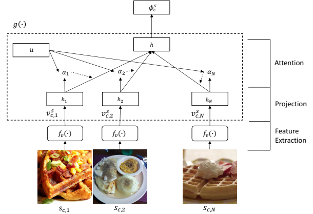
Figure 2. Reference set encoder f_s(\cdot)
