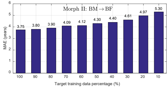
Figure 5. The cross-population age estimation results w.r.t. the percentage of the training data in the target population.
