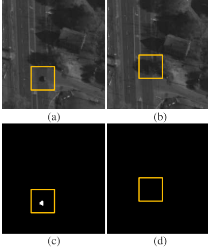
Figure 3. Illustration of why trackers based on moving object detection fail. (a) and (b) are consecutive frames with the yellow box showing the location of the object. (c) and (d) are the binary images of (a) and (b) respectively, showing moving objects in the scene. The object of interest is completely lost in (d) since it moved into the shadow region.
