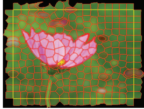
Figure 2. Illustration of the absorbing nodes. The superpixels outside the yellow bounding box are the duplicated boundary superpixels, which are used as the absorbing nodes.
