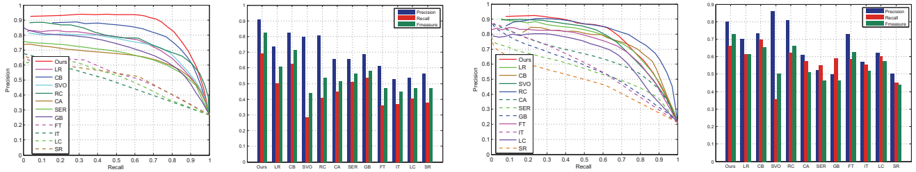
Figure 6. Evaluation results on the SED dataset. Left two: the results for different methods on the SED1 dataset. Right two: the results for different methods on the SED2 dataset.
