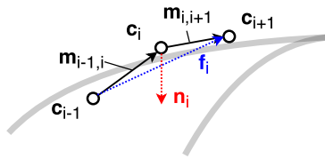
Fig. 3. Estimation of the road normal \mathbf{n}_i and forward direction \mathbf{f}_i at a single frame i . The final estimate is an aggregate over all frames.
