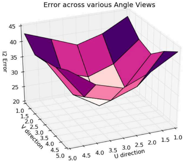
Figure 5. Error in Angular Viewpoints: Here we visualize the \ell_2 error for a light field reconstruction with respect to ground truth using a standard \ell_2 loss function for training. Notice how the extreme angular viewpoints contain the highest error. This helped motivate the use of a weighted \ell_2 function for training the network.
