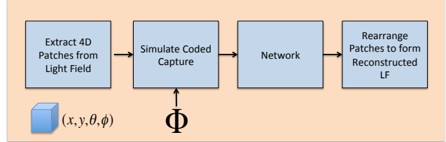
Figure 2. Pipeline: An overview of our pipeline for light field reconstruction.
