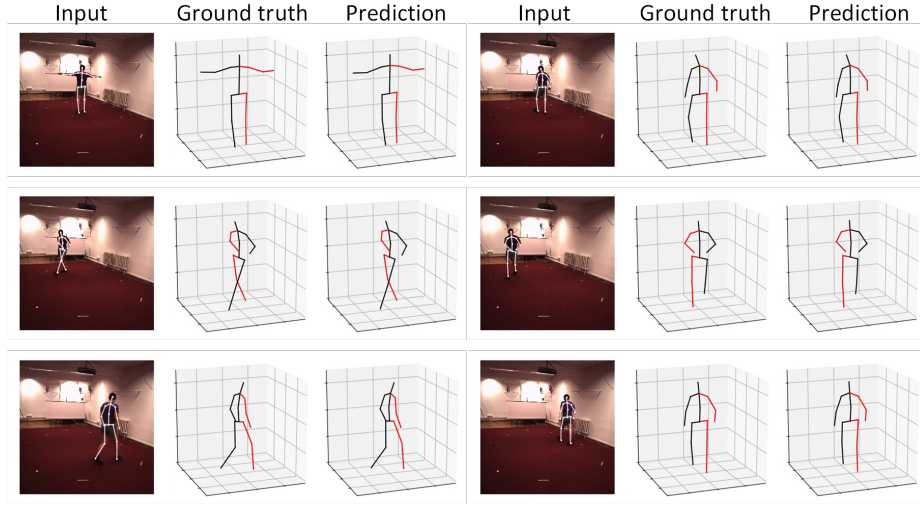
Fig. 7. Some qualitative results of our approach on Human3.6M.
