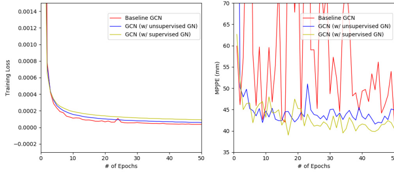
Fig. 5. The trend of the 3D HPE loss and the validation MPJPE during training. The number of parameters of each model is approximately 2.69M. Unsupervised GN means the global node output is directly discarded in the training phase while supervised GN means the global node is supervised by action labels generated by K-means.
