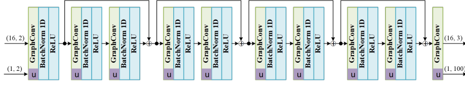
Fig. 4. This figure shows the GCN architecture we apply in our experiments. The building block is a residual block composed of two graph convolutional layers with 128 channels. This block is repeated four times. Each graph convolutional layer (except for the last one) is followed by a batch normalization layer and a ReLU activation layer.
