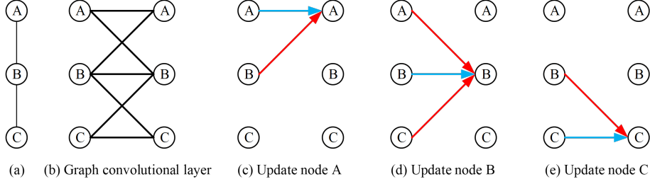
Fig. 2. Illustration of the feature update in a graph convolutional layer. Blue arrows and red arrows respectively correspond to self-connections and other-connections. (a) A simple graph consisting of three nodes. (b) The updated features of each node (the right side) depend on the input features of itself and its neighboring nodes (the left side). (c)(d)(e) respectively show the feature update of nodes A, B and C.
