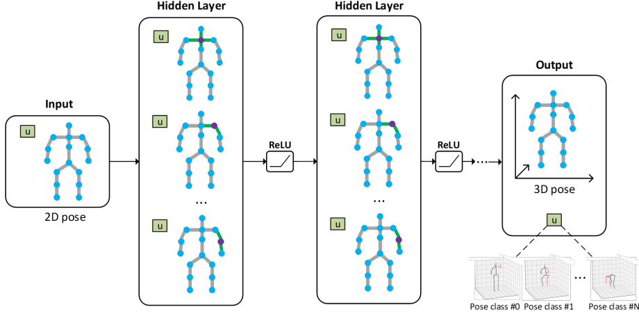
Fig. 1. Illustration of a graph convolutional network (GCN) with a global node u for 3D human pose estimation. The input is the 2D body joint locations predicted by an off-the-shelf 2D pose detector with a zero-initialized global feature vector. The GCN repeatedly transforms and aggregates features of local and global nodes to learn increasingly powerful representations. Finally, it predicts the 3D pose as well as the output of an auxiliary task, e.g., an action label of the pose.
