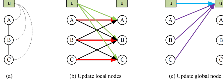
Fig. 3. Illustration of the feature update for local nodes and the global node. Arrays of the same color means applying the same weight matrix. (a) A simple graph composed of three nodes: A, B and C. u is the added global node, which is connected to all local nodes. (b) The feature update of local nodes. (c) The feature update of the global node.
