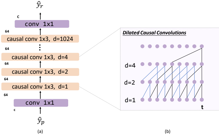
Fig. 4. (a) An overview of causal TCN, which can be performed online. The dilation factor is doubled at each causal layer, i.e. 1, 2, 4, ..., 1024. (b) The architecture of the causal convolutions with different dilation factors.
