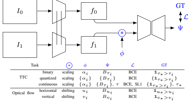
Figure 4: Architecture. We perform all of our tasks with minor modifications to the same backbone. We preprocess the input images by extracting features and applying a task dependent operation, (*) , to the features of the second image. The input parameter \phi , the loss, \mathcal{L} , the ground truth, GT, and the output, \Psi for each task are listed in the table. Note that \{\cdot\} indicates a set, and \mathbb{1} the indicator function.
