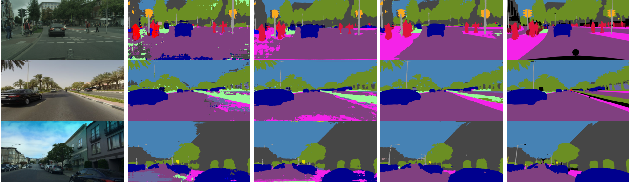
Figure 4. Qualitative illustration of domain generalizable semantic segmentation for GTA5 to Cityscapes (1st row), Mapillary (2nd row), and BDD (3rd row). FSDR preserves domain invariant information during domain randomization which produces better semantic segmentation especially around edge/class-transition area. As a comparison, DRPC [77] does not isolate and preserve domain invariant feature which leads to sub-optimal segmentation.
