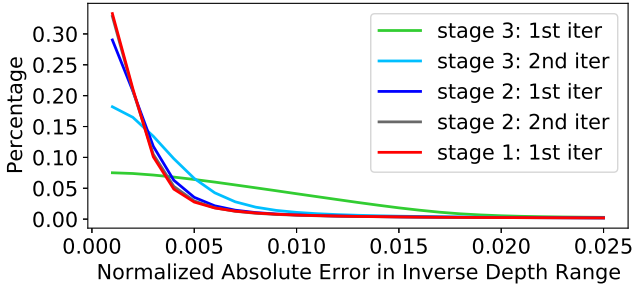
Figure 9: Distribution of normalized absolute errors in the inverse depth range on DTU’s evaluation set [1]. ‘Stage k , n th iter’ denotes the result of the n th iteration of Patchmatch on stage k . Already after stage 3 our estimate is close to the solution while stage 2 and 1 refine it even more.
