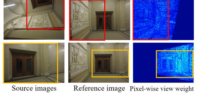
Figure 8: Visualization of our pixel-wise view weight on a scene from ETH3D [30]. Areas marked with boxes in source images and reference image are co-visible. Right: The corresponding pixel-wise view weights, bright colors (large values) indicate co-visibility.
