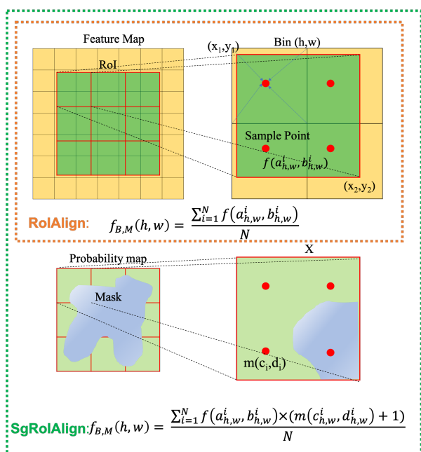
Figure 1: A diagram of shape-guided RoIAlign.
