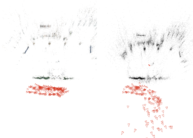
Figure 5. Failure Case. The figure shows a failure case in the Lobby scene where focal lengths are increasingly overestimated. The reference model from keypoints and with known camera parameters ( Left ) vs. the failed reconstruction from lines with unknown camera parameters ( Right ). The wrong focal lengths cause the images to be placed further back.
