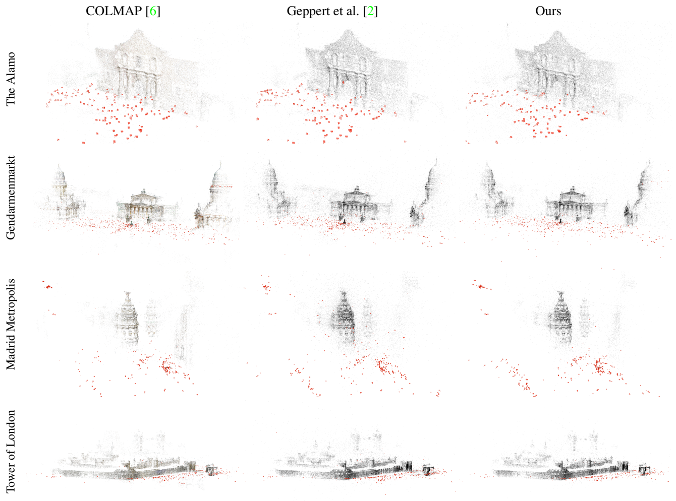
Figure 6. Qualitative Results. Comparison between standard COLMAP [6] ( Left ), the calibrated privacy preserving SfM from Geppert et al. [2] (using known intrinsic calibration, Middle ), and our uncalibrated privacy preserving reconstruction pipeline ( Right ). Note that the reconstruction results depend on multiple parameters/thresholds which might not be comparable between the methods.
