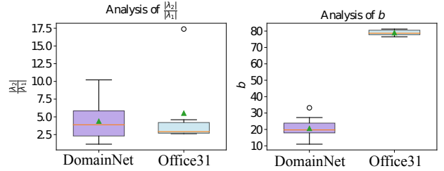
Figure 4. Analysis of learned coefficients.
