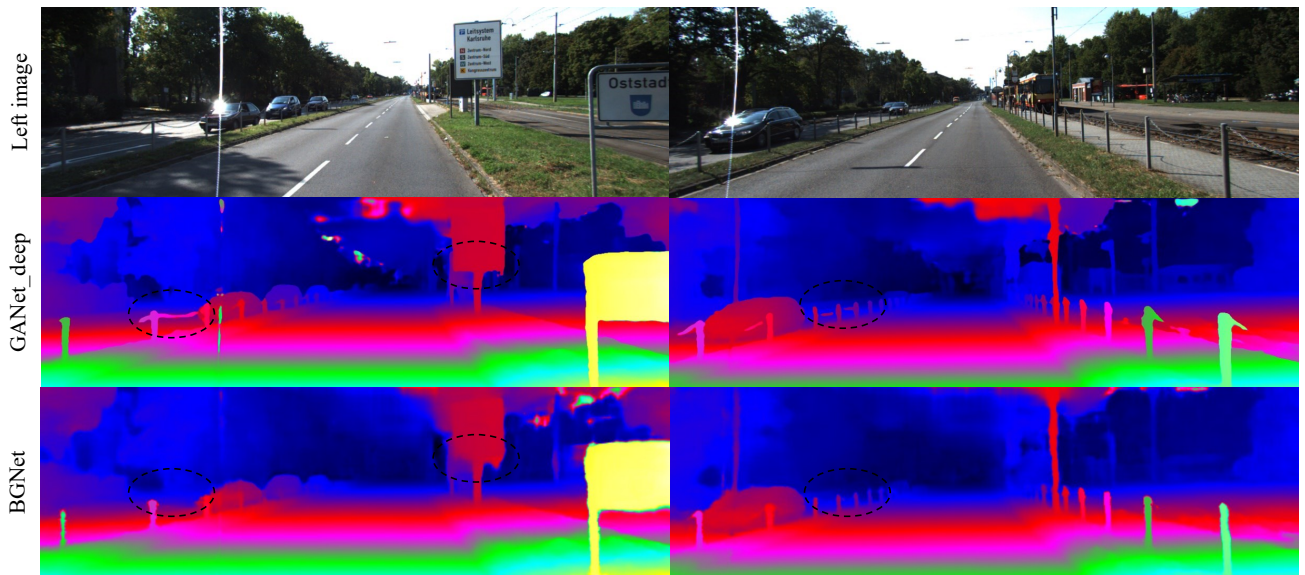
Figure 1. Failure cases of BGNet on the KITTI 2015 dataset
