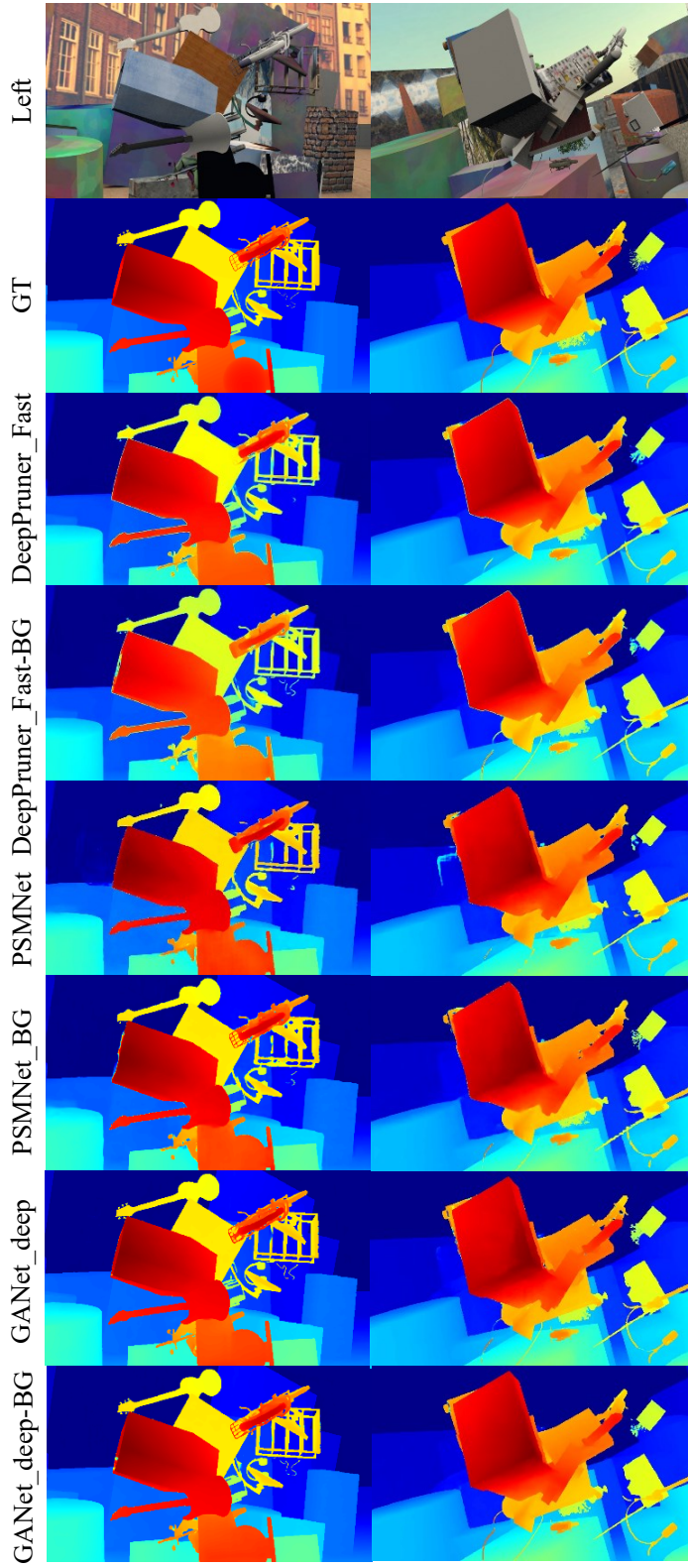
Figure 2. Qualitative results of the existing networks, before and after adding the BG module.
