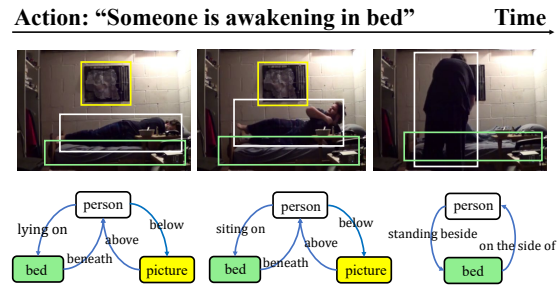
Figure 1. An illustration example from Action Genome [22]. It demonstrates that actions can usually be decomposed into evolving spatio-temporal scene graphs ( i.e. , how a person interacts with surrounding objects over time such as person-lying-on-bed to person-sitting-on-bed ). Inspired by this, we propose to use a data-driven Markov Logic Network to model this evolving pattern.
