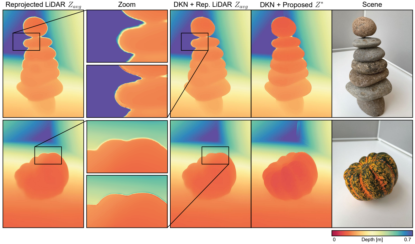
Figure 9: RGB-guided depth upsampling methods use a high-resolution RGB image as guidance for the superresolution and refinement of potentially noisy depth data. These leverage the prior that depth and color changes are often highly correlated to produce visually consistent high-resolution depth outputs. We find that for our data that DKN can use this correlation to improve the reconstruction of sharp depth edges, matching them to the edges of objects in the image, as seen in the zoomed views above. This can often correct for the edge blurring caused by occlusions as discussed in Section 2.6. However, as RGB-guided upsampling does not take parallax effects into account, this approach cannot extract any new depth features that were not already present in the underlying data. Correspondingly, areas not along an edge see very little change in depth after the application of DKN.
