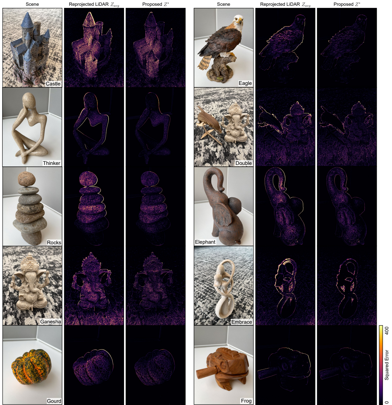
Figure 4: Visualization of squared photometric error PE , as defined in Section 5 of the main text. We see that nearly all the photometric error is accumulated from the high image contrast areas (e.g. object borders and large color features). This matches our previous intuition, as these are the regions our proposed method refines. We see a significant reduction in error around depth discontinuities, such as around the borders of the objects, as well as intra-object features such as the feathers of eagle , the central curves of gourd , and the body of ganesha .
