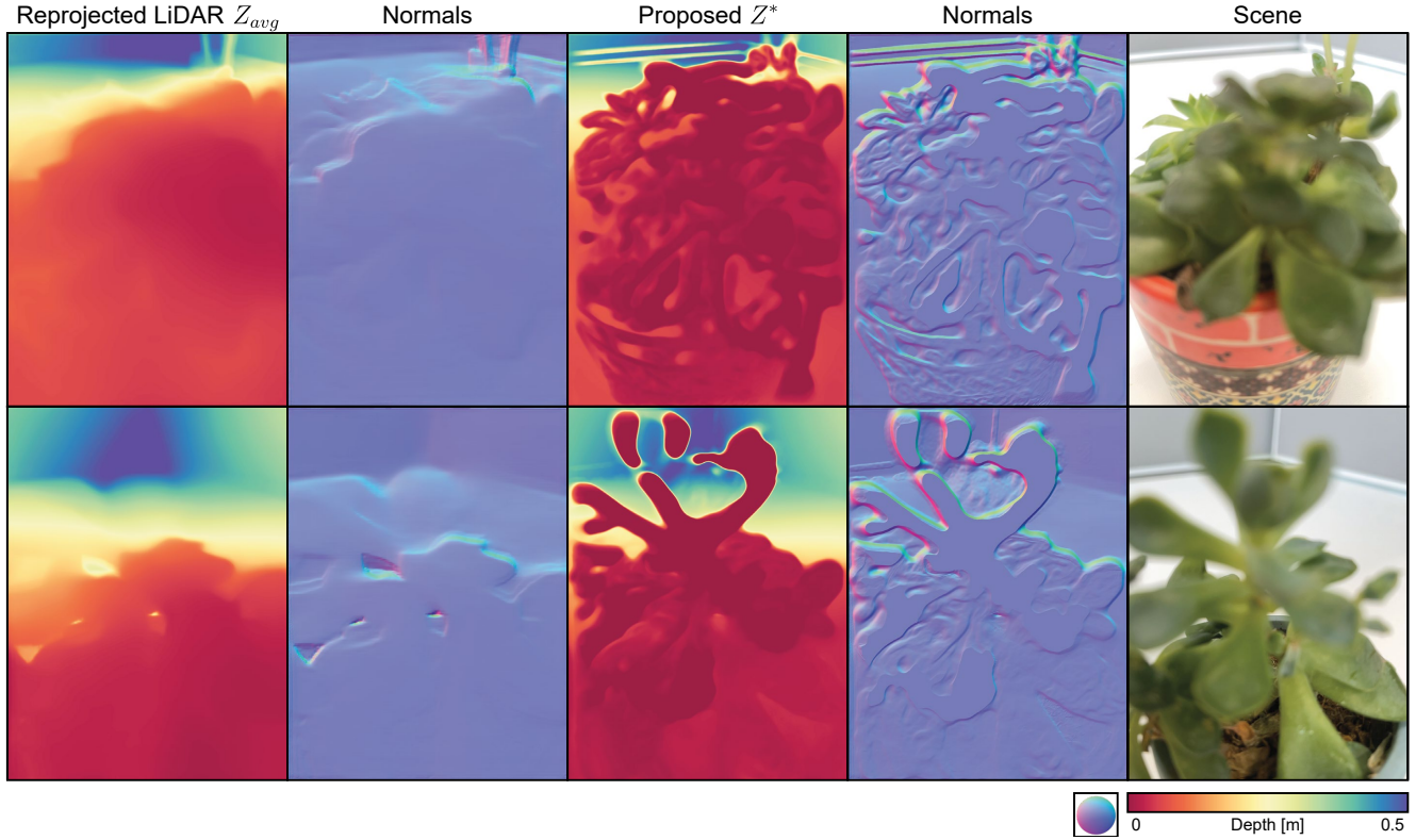
Figure 6: While closer-range objects provide better parallax cues from which to reconstruct depth, our phone has a minimum focus distance of approximately 8cm. Objects closer than this exhibit significant lens blur as can be seen in the scene photos above. In this regime, useful photometric information is overpowered by lens distortions and the now mixed background and foreground pixel colors. While our method can recover depth features for in-focus regions (e.g. the flower pot and lower petals), neither our method nor the underlying LiDAR depth data is able to produce reliable depth for regions under extreme blur. In practical application we expect this to be a rare edge case as a phone photographer is unlikely to capture a snapshot of scene which is clearly blurry in the viewfinder. One potential workaround, implemented by many popular camera applications, is to produce a notification which urges the user to “move back to improve focus”.
