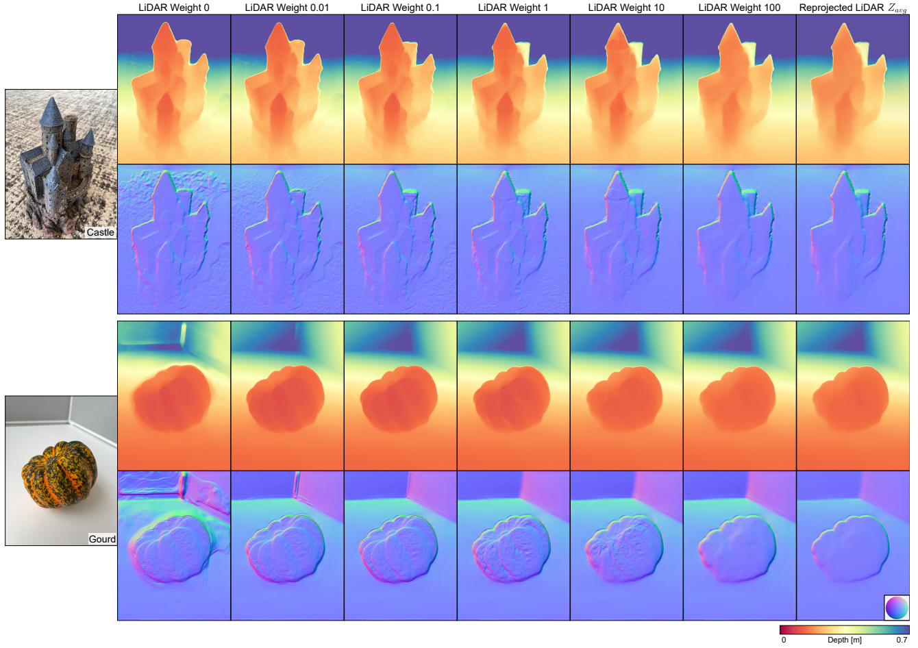
Figure 11: Reconstruction results for varying geometric regularization weight \alpha . With no geometric regularization term ( \alpha = 0 ) we see that the depth reconstruction of the textureless object backgrounds erroneously drift away from the underlying LiDAR data as there is no guiding photometric loss in those regions. When \alpha is non-zero, these textureless regions are effectively locked to the LiDAR depth solution. As we increase \alpha , the overall reconstruction is pulled closer to the LiDAR depth, with the reconstructed depth for \alpha = 100 being virtually identical to the reprojected LiDAR depth Z_{avg} . As we desire a reconstruction almost entirely guided by micro-baseline photometric information, to fix LiDAR depth artifacts like those at the top of the castle example, we choose a small \alpha = 0.01 .
