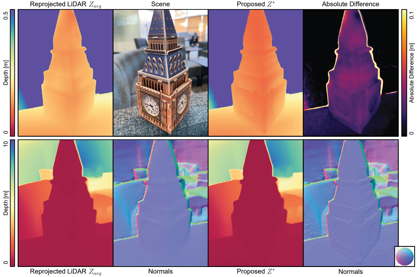
Figure 7: In this scene we have an object resting on a couch arm approximately 15cm away from the phone, with the background content of the room extending 8+ meters into the distance. We note that the short focus distance also noticeably blurs these distant regions. Similar to what is observed in Figure 6, the depth of the background regions remains unperturbed, as it provides virtually no meaningful photometric information. At the same time, the foreground object is successfully reconstructed and we recover fine geometric features such as bumps and protrusions on the surface of the replica clock-tower. This demonstrates that our method, by virtue of its design alone, refines close-range objects without adversely affecting their un-refineable surroundings.
