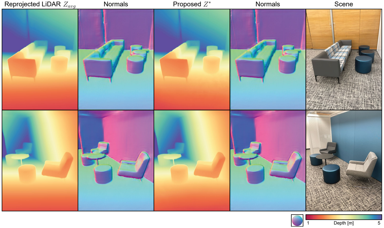
Figure 5: As outlined in Section 4 of the main text, even well-textured objects at depths of greater than 1 meter produce sub-pixel disparities for a micro-baseline stereo setup. In this scenario there is insufficient photometric guidance to reconstruct any new depth features, and our results gracefully degrade to the averaged LiDAR depth output. As we learn depth offsets \Delta z rather than the direct depth z , our model can trivially output no offset – unperturbed by the minimal photometric loss.
