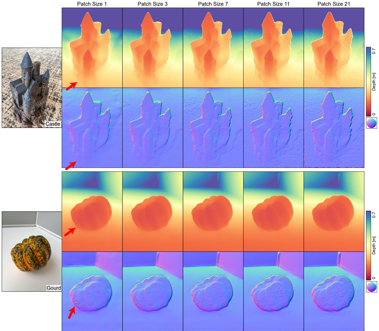
Figure 10: Reconstruction results for varying patch size K . Note the depth artifacts, highlighted with red arrows, where single-pixel photometric information is insufficient to correctly resolve depth, and false matches drive the reconstruction to find incorrect local minima solutions. As we increase patch size these artifacts disappear, but we also fatten the reconstructed object edges and can blur thin structures. Patch size 11 achieves a reasonable mezzanine between artifact suppression and fine feature reconstruction.
