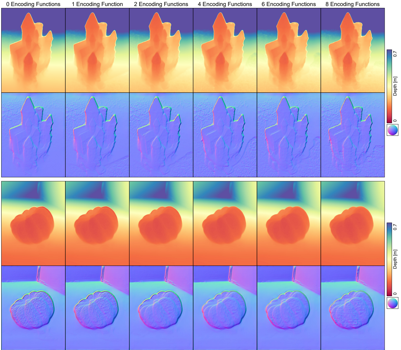
Figure 12: Reconstruction results for varying encoding function count L . We see that without positional encoding, for L = 0 , our reconstruction is quite noisy and does not correct for the depth artifact at the top of the castle example. We speculate the MLP overfits to RGB and depth information in this case, rather than learning true corrective offsets for depth refinement. At L = 8 encoding function we start to see high frequency artifacts bleed into the reconstruction. We thus choose L = 6 functions as a reasonable mezzanine where neither of these effects are present.
