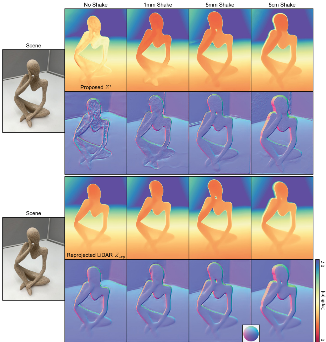
Figure 8: As discussed in Section 1.2 of this supplemental document and Section 4 of the main text, the maximum effective baseline of a recorded bundle is important in determining what we are able and unable to reconstruct. As seen above, with a static camera (and thus an effective baseline of 0mm), there is not only insufficient parallax information from which to reconstruct new depth features, but nearly all the information we do have is incorrect. Small errors in the pose estimation algorithm dominate the overall signal, and we reconstruct incorrect and noisy depths. As we increase the effective baseline to 1mm we see the effects of this noise diminish, however there still appear to be depth artifacts where we find incorrect local minima solutions due to the small view variation. At 5mm we see recovery of fine depth details consistent with Figure 3 and results in the main text, this is what is considered an example of a good hand shake . When the effective baseline is further increased to 5cm (closer to a typical stereo camera setup), we see some improvement in reconstruction of fine features such as the model's feet, however both our and the reprojected lidar depth produce a large number of flying pixels around the edges of the statue. This is due to the fact that neither model can explicitly handle occlusions, and instead mix foreground and background depths around discontinuities.
