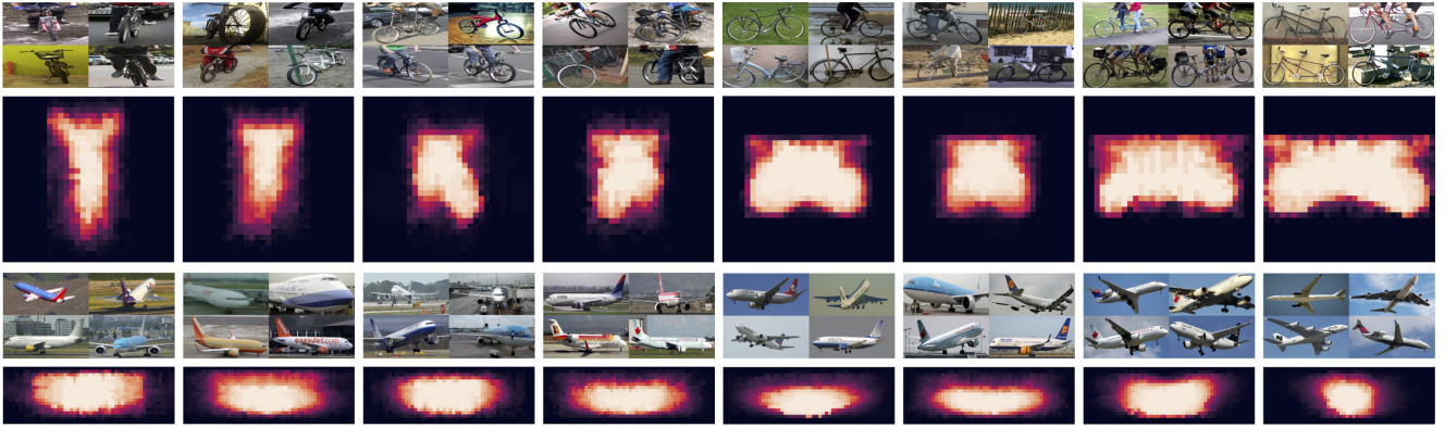
Figure 1: Additional Compositional Spatial Priors Visualizations. M = 8 spatial priors belonging to the bicycle and aeroplane class are shown. Each prior P(\vec{w}|y, m) is displayed below the examples of its corresponding learned objects.
