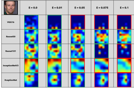
Figure 5. Black box attack example, depicting the shifting behaviour in the region of participating as \epsilon increases
