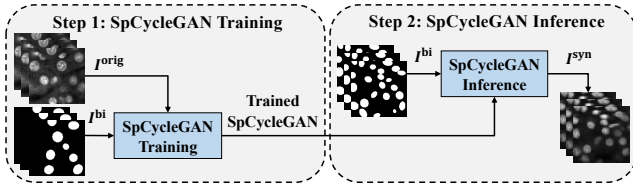
Figure 3. 3D synthetic microscopy volume generation using SpCycleGAN
