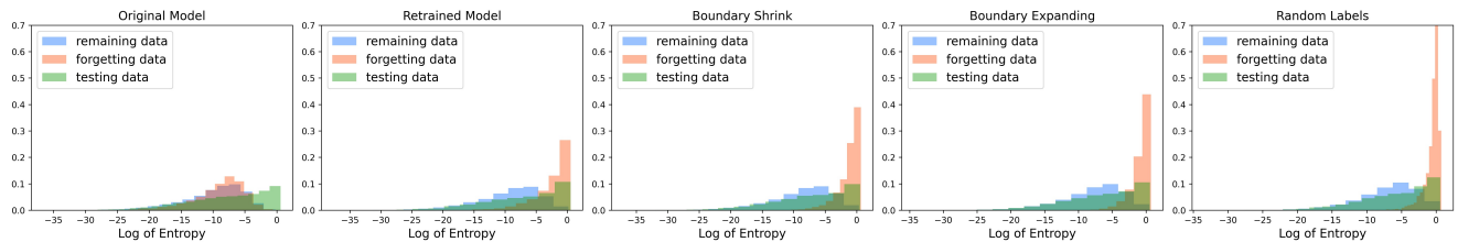
Figure 7. Distribution of the entropy of model's output on the remaining data \mathcal{D}_r , the forgetting data \mathcal{D}_f and the testing data.
