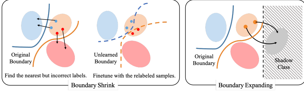
Figure 2. Illustrating the key ideas of Boundary Shrink and Boundary Expanding. The ovals in different colors represent features of samples in different categories and the dots represent the training samples of the forgetting class. Both Boundary Shrink and Boundary Expanding can destroy the decision boundary of the forgetting class.
