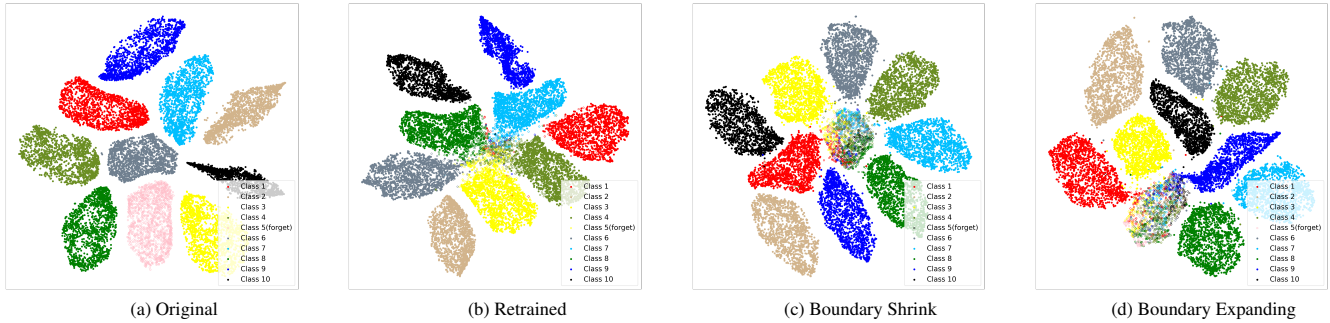
Figure 6. Visualization of decision space of different methods on CIFAR-10 dataset. The solid dots in different colors represent samples belonging to different remaining classes and the hollow circles stand for the forgetting data. Ideally, we wish the unlearned models act like the retrained model.
