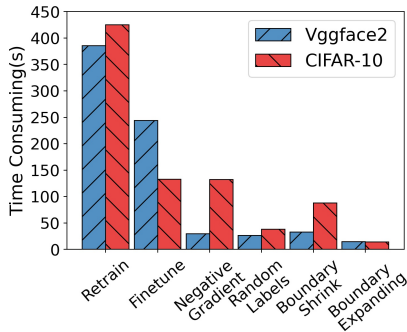
Figure 4. The time consumption of each unlearning method.
