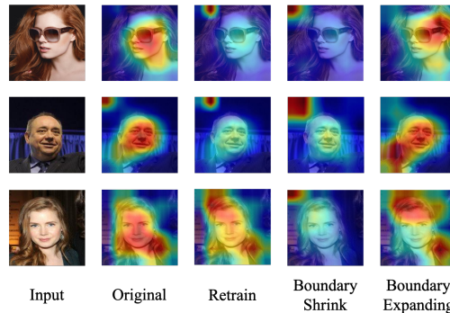
Figure 5. The attention map of each unlearning method.
