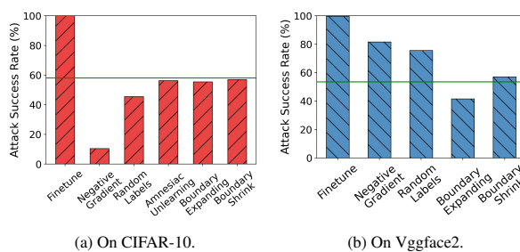
Figure 3. The attack success rate of each unlearning method. The green line represents the ASR of the retrained model, and it is expected to be more close to it to reduce the privacy leakage.
