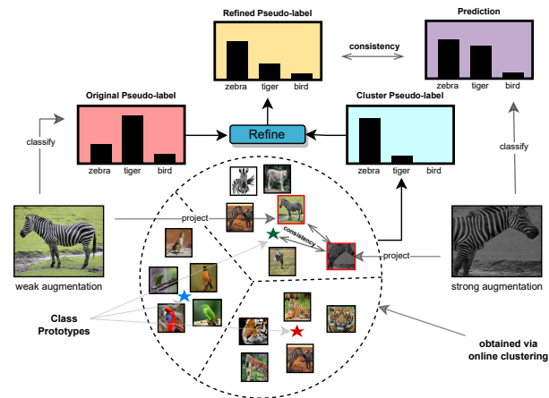
Figure 1. PROTOCON refines a pseudo-label of a given sample by knowledge of its neighbours in a prototypical embedding space. Neighbours are identified in an online manner using constrained K-means clustering. Best viewed zoomed in.
