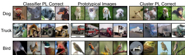
Figure 4. The middle panel shows the most prototypical images of CIFAR-10 classes as identified by our model. Left (resp. right) panels show images which have more accurate classifier (resp. cluster) pseudo-labels. Cluster labels are more accurate for prototypical images while classifier labels are more accurate for images with distinctive features (e.g. truck wheels) even if not so prototypical. Such diversity of views is key to the success of our co-training method.
