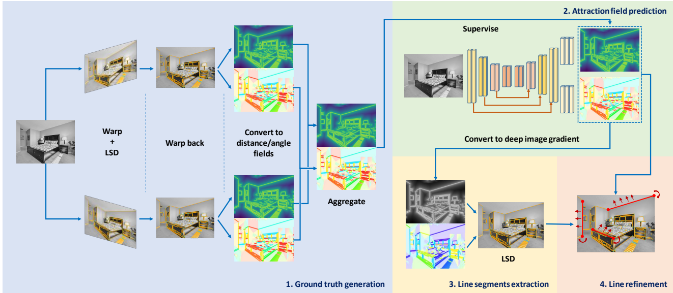
Figure 2. Overview of the method. (1) We generate ground truth line distance and angle fields (DF/AF) by bootstrapping LSD [51]. (2) A deep network is trained to predict the DF/AF, which is then converted to a surrogate image gradient. (3) Line segments are extracted with LSD and (4) refined based on the DF/AF.
