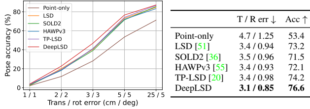
Figure 7. Visual localization on 7Scenes stairs [47]. We evaluate the median translation and rotation errors (cm / deg), the pose accuracy at a 5 cm / 5 deg threshold, and plot the pose accuracy curve for various thresholds.
