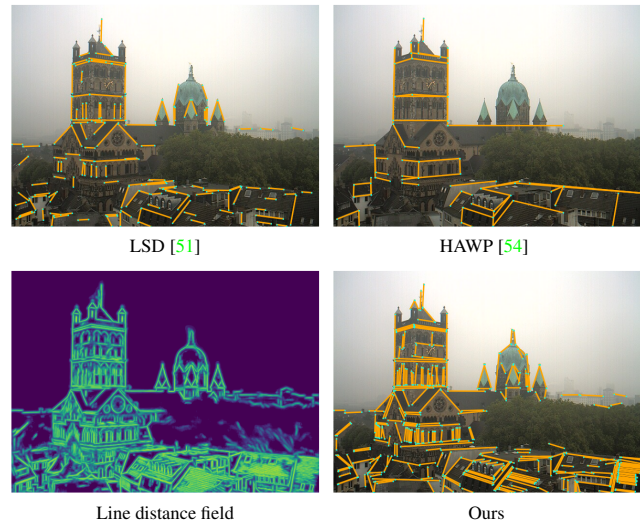
Figure 1. Line detection in the wild. Top row: on challenging images, handcrafted methods such as LSD [51] suffer from noisy image gradients, while current learned methods like HAWP [54] were trained on wireframe images and generalize poorly. Bottom row: we combine deep learning to regress a line attraction field and a handcrafted detector to get both accurate and robust lines.
