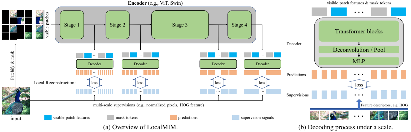
Figure 2. Illustration of local multi-scale reconstruction. a) We randomly mask some input patches and then predict their supervision signals of different scales at multiple local layers. The multi-scale supervisions are obtained by first dividing the input under different scales and then extracting signals with some feature descriptors. The lower layers are responsible for fine-scale reconstruction and the upper ones are responsible for coarse-scale reconstruction. We also use the asymmetric encoder-decoder strategy for quick encoding. b) The decoder consists of three parts: Transformer blocks, Deconvolution/Pool (optional) and Multilayer perceptron.
