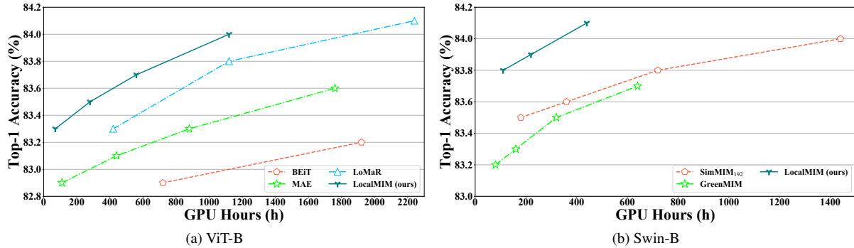
Figure 1. Top-1 fine-tuning accuracy on ImageNet-1K vs. Pre-training duration. The duration is estimated on a machine with one Tesla V100-32G GPU, CUDA 10.2 and PyTorch 1.8. ‘GPU Hours’ is the running time on single GPU.
