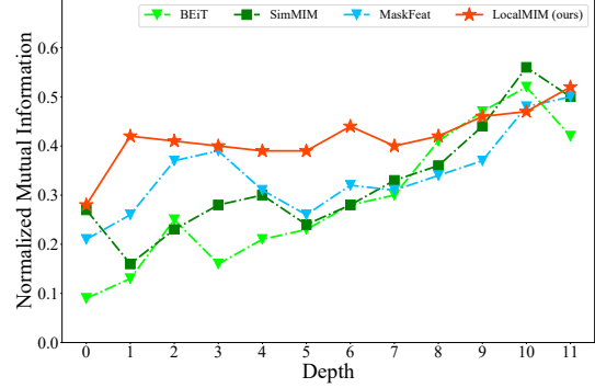
Figure 3. Normalized Mutual Information (NMI) between query and key patches at each layer of a pre-trained ViT-B.
