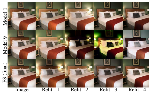
Figure 4. The bottom row shows scene relightings obtained using our final, forward selected, set of directions (star of Figure 3). For comparison, we also show scene relightings from different models obtained from StyLitGAN shown in Figure 3 (model numbers correspond to numbers on that figure). Note how most models are capable of producing some good directions, but not all directions from a given model may be good.
