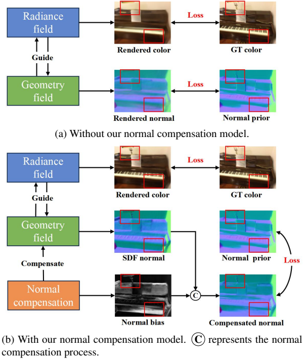
Figure 3. Visualization of rendered results , comparing (a) without and (b) with our normal compensation model. \odot represents the normal compensation process.
