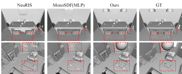
Figure 6. Qualitative results on ICL-NUIM [17].
