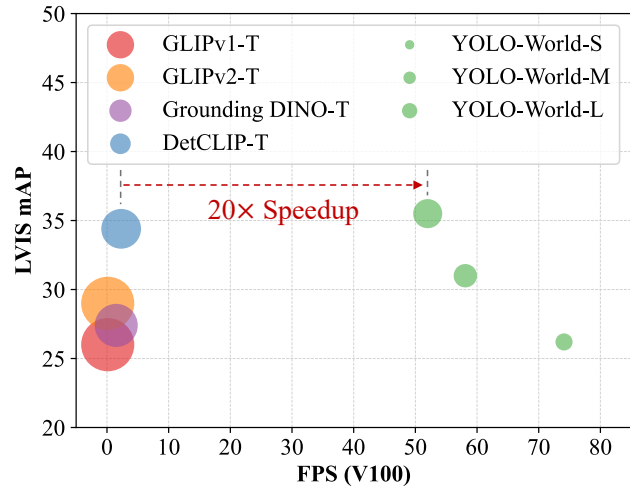
Figure 1. Speed-and-Accuracy Curve. We compare YOLO-World with recent open-vocabulary methods pre-trained similar datasets ( i.e. , Objects365 [46] and GoldG [21]) in terms of speed and accuracy. All models are evaluated on the LVIS minival (using Fixed AP [4]) and inference speeds are measured on one NVIDIA V100 w/o TensorRT. The size of the circle represents the model’s size.
