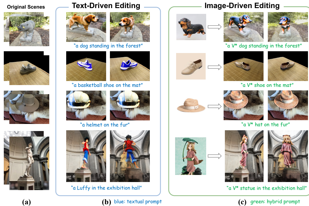
Figure 1. Adaptive source driven editing by CustomNeRF. Our method can accurately edit the original NeRF scene according to text descriptions or reference images, which are formulated as textual prompts or hybrid prompts. After editing, the foreground regions exhibit appropriate geometric and texture modifications consistent with the editing prompts. The layouts and background contents of the edited scenes remain almost the same as the original ones.
