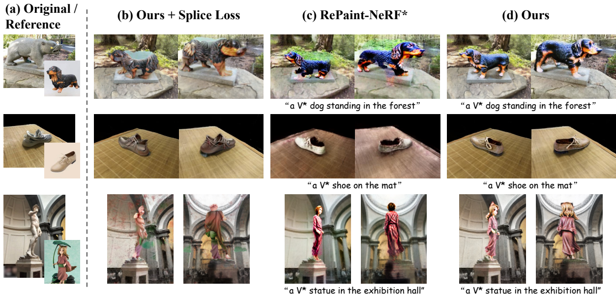
Figure 3. Qualitative comparison on the image-driven editing setting. * denotes replacing the employed T2I model with Custom Diffusion.
