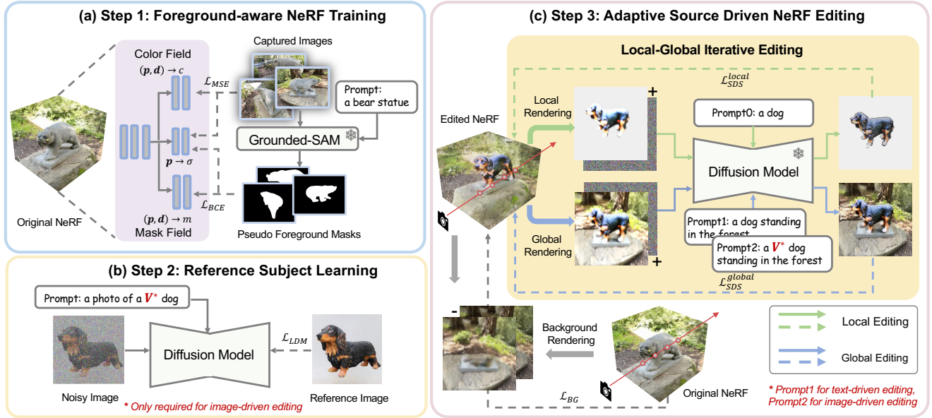
Figure 2. The overall pipeline of our CustomNeRF. Given an original 3D scene, CustomNeRF aims to edit it according to a textual description or a reference image. Our pipeline consists of three steps in total. (a) Reconstruct the original 3D scene with a foreground-aware NeRF, which enables the identification of foreground regions. (b) Finetune the pre-trained text-to-image diffusion model to embed the visual subject in the reference image into a special token V^* . This step is only required in image-driven editing. (c) Optimize the given NeRF with our proposed Local-Global Iterative Editing (LGIE) training scheme to align with the textual description or the reference image. The local and global data flows occur in an alternating manner. Prompt2 is employed in image-driven editing whereas Prompt1 is utilized in text-driven editing. Prompt0 is shared in both editing settings.
