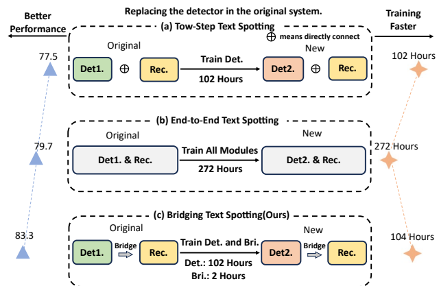
Figure 1. Comparison between the proposed paradigm with existing text spotting paradigms. Our pipeline achieves better performance with high modularity. We adopt the latest detector [66] and text spotter [62] to test the training time of the two-step and end-to-end methods, respectively. The training time is evaluated on the RTX-3090. Det1. means the original detector. Det2. means the new detector. Rec. means the text recognizer. Bri. mean the proposed Bridge.
