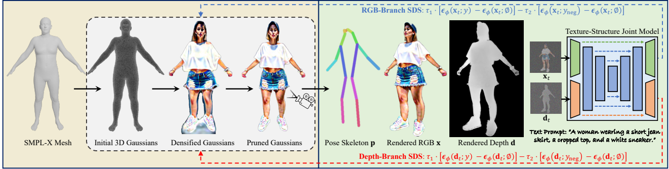
Figure 2. Overview of the proposed HumanGaussian Framework. We generate high-quality 3D humans from text prompts with the neural representation of 3D Gaussian Splatting (3DGS). In Structure-Aware SDS , we start from the SMPL-X prior to densely sample Gaussians on the human mesh surface as initial center positions. Then, a Texture-Structure Joint Model is trained to simultaneously denoise the image \mathbf{x} and depth \mathbf{d} conditioned on pose skeleton \mathbf{p} . Based on this, we design a dual-branch SDS to jointly optimize human appearance and geometry, where the 3DGS density is adaptively controlled by distilling from both the RGB and depth space. In Annealed Negative Prompt Guidance , we use the cleaner classifier score with an annealed negative score to regularize the stochastic SDS gradient of high variance. The floating artifacts are further eliminated based on Gaussian size in a prune-only phase to enhance generation smoothness.
