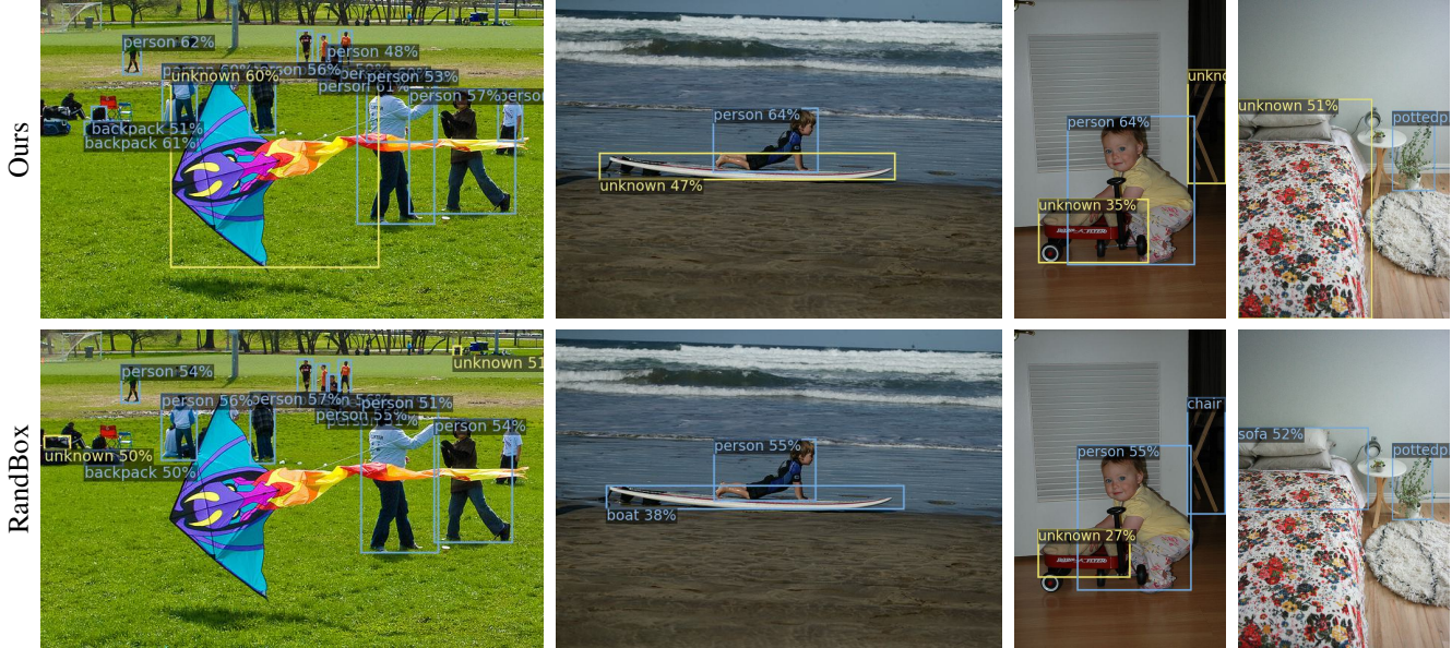
Figure 5. Qualitative results on M-OWODB. We compare with a leading open world object detector RandBox [71] in terms of known and unknown object detections after the second stage of M-OWODB. Each image pair uses the same score threshold for a fair comparison.
