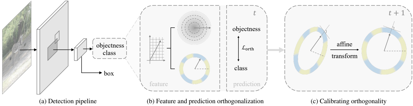
Figure 2. Overview of the proposed method for open world object detection. (a) We build on a Fast R-CNN [17] based architecture, and employ three levels of orthogonality to mitigate interference between objectness and class predictions. (b) Specifically, the feature of each object proposal is decomposed under a polar coordinate system for separate predictions, followed by a regularization loss that further decorrelates these predictions. (c) During the learning process, we also incorporate affine transforms to continually calibrate orthogonality.
