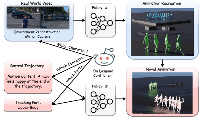
Figure 3. Our framework presents an on-demand control system tailored for real-world videos. Beginning with the pre-processing in [60], our policy network can track high-confidence motions and effectively fill in missing parts without additional fine-tuning. Moreover, our framework offers the novel functionality of introducing customized animations into real-world scenarios with flexible control options.
