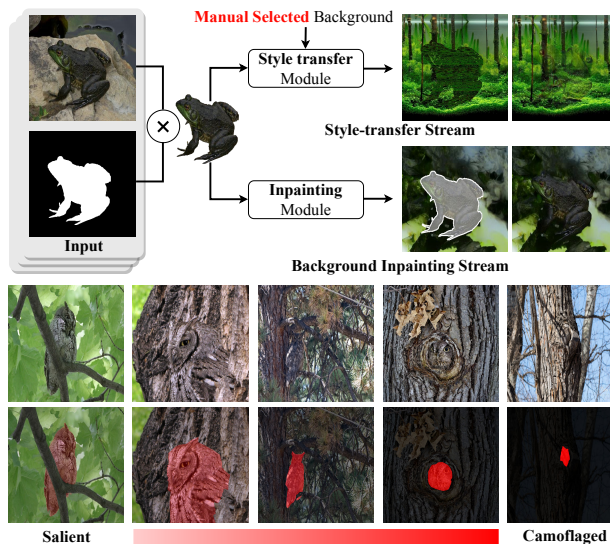
Figure 2. Comparison of Frameworks for Camouflage Image Generation. Existing methods rely on manually specified backgrounds, which not only receive limitations in diversity and scope from the human’s own cognition but also result in expensive image generation on a large scale. Without changing the texture of itself, the same target can be camouflaged to different degrees in different environments. Inspired by it, we synthesize camouflaged images through a background inpainting stream, hiding by automatically choosing a suitable background for the object.
