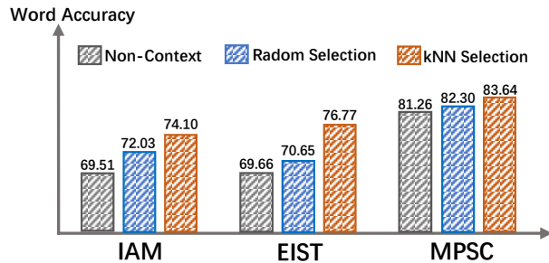
Figure 6. Comparison between different in-context prompt selection strategies. ‘‘Random Selection’’ refers to randomly selecting two samples as in-context prompts from the in-context pool. X-axis is the evaluated benchmarks.
