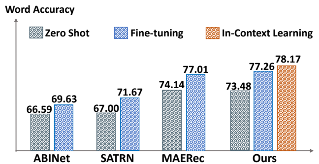
Figure 5. Comparison with the fine-tuned models. We report the average performance on three cross-domain datasets. Please note that ABINet [10], SATRN [20] and MAERec [17] are fine-tuned with the in-domain data, while our E 2 STR-ICL is training-free.
