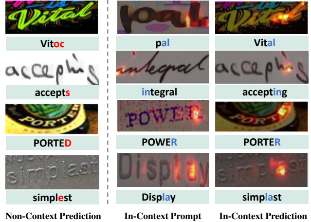
Figure 8. Cross attention visualization between the language tokens and the vision tokens. Left: Non-context prediction of E 2 STR. Error characters are marked in red. Right: In-context prediction of E 2 STR-ICL, where only one in-context prompt is selected. We visualize how the language tokens attend to the prompt image and the test image.
