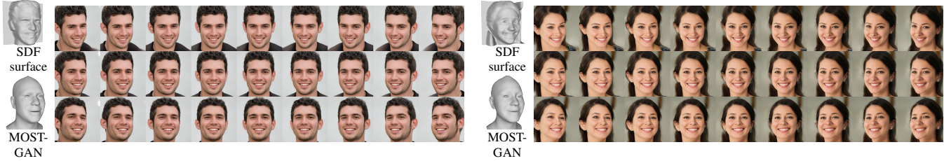
Figure 3. Multiview image renderings and 3D shapes using marching cubes from CoLa-SDF as well as MOST-GAN reconstructions. Please zoom-in for details.
