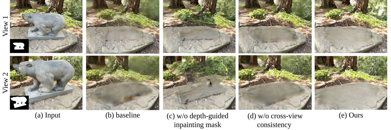
Figure 7. Ablation studies on the Bear scene from the InNeRF360 [34] dataset. We verify the effectiveness of our Inferring Depth-Guided Inpainting Mask and Inpainting-guided 3DGS Refinement.
