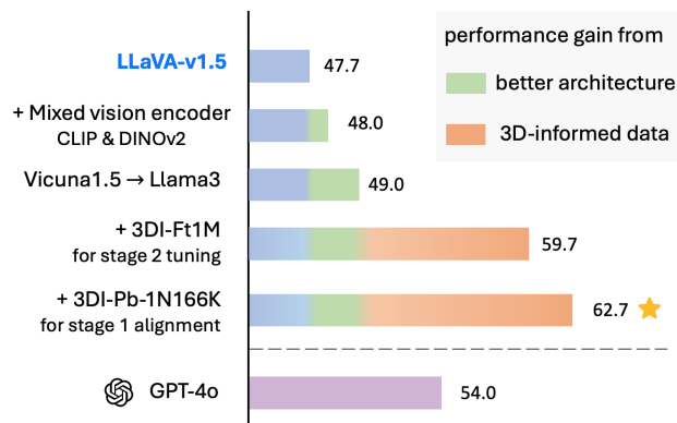
Figure 6. We modernize a standard LLaVA-v1.5 towards the design of a 3D-informed LMM. The bars are the answer accuracies on the SpatialVQA benchmark, indicating the spatial reasoning capability of each model; results for the GPT-4o is shown with the purple bar.
