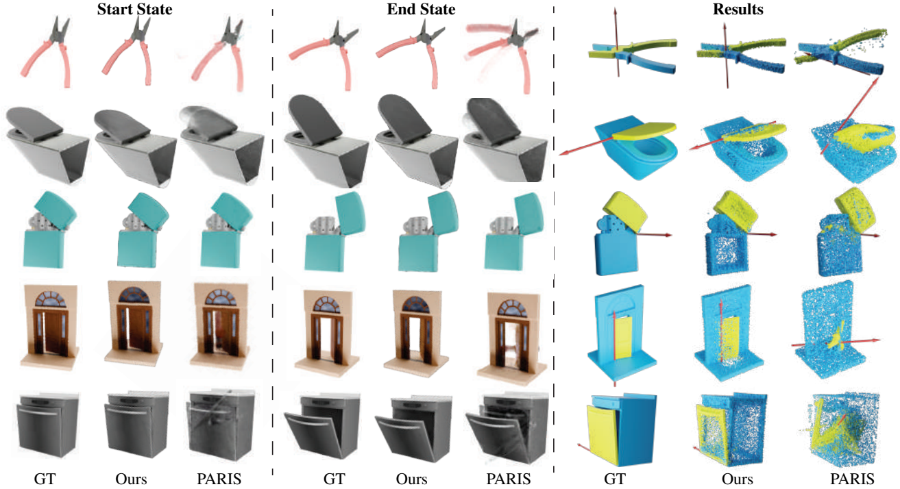
Figure 2. Illustration of the effects of applying our method and the PARIS algorithm to our dataset. It includes the appearance at the beginning and end states, along with part segmentation and motion estimation for both methods.
