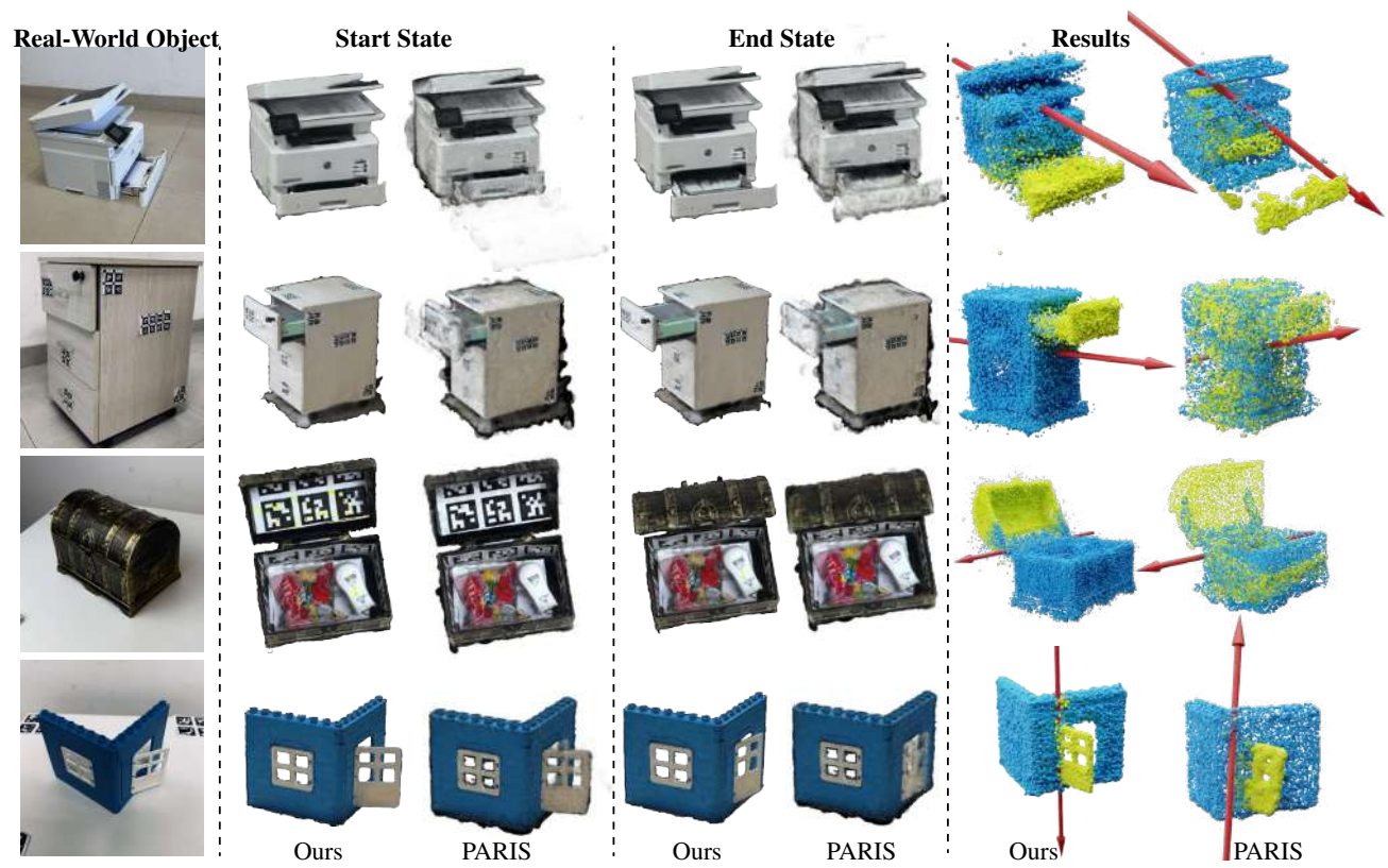
Figure 3. Illustration of applying our method and the PARIS algorithm to real-world objects.
