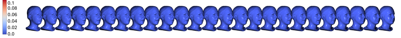
(b) VOCA [11].
