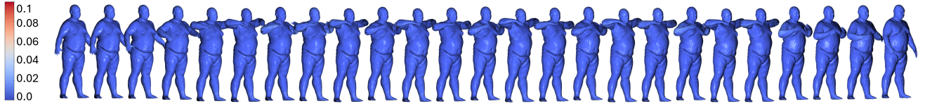
(c) DFAUST [6].
