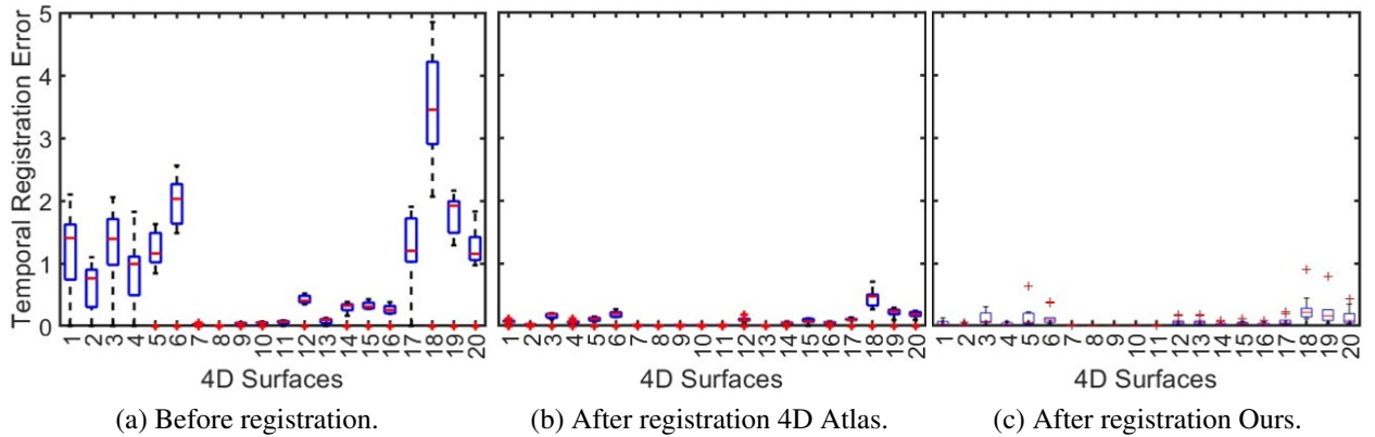
Figure 17. Boxplot visualization of the spatiotemporal registration experiment performed in Figure 8 in the main manuscript. We show the alignment error (a) before spatiotemporal registration, (b) after spatiotemporal registration using 4D Atlas [19], and (c) after spatiotemporal registration using our framework.
