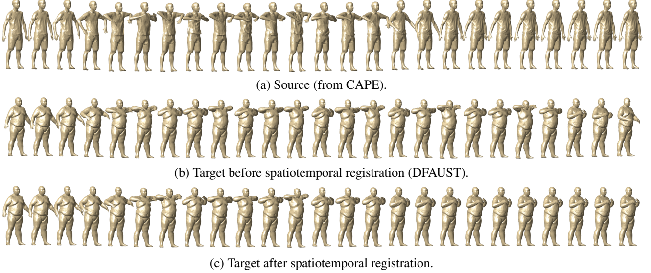
Figure 14. An example of the spatiotemporal registration of 4D humans performing an action across two datasets. We show an example of the CAPE and DFAUST dataset, with different discretizations and correspondences.
