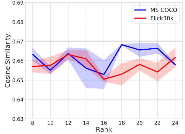
Figure 6. Cosine similarity across different TT ranks on COCO and Flick30k datasets.
