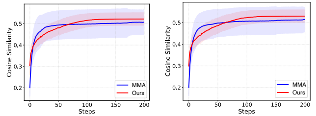
Figure 7. Convergence comparison between our sequential probability tensor estimation and MMA (using coordinate-wise GCG [46]) on MS COCO and Flick30k datasets.
