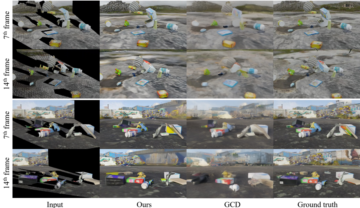
Figure 3. Qualitative results on Kubric4D [5]. Compared to GCD [10], our method demonstrates superior performance in preserving object details and dynamics in input videos.
