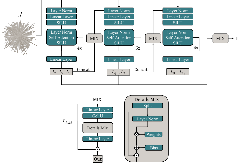
Figure 1. (Top) Overview of all the blocks involved in the digital encoder architecture. The three steps capture coarse, middle, and fine details, with each step depending on the output of the previous one. (Bottom) Illustration of the MIX process. The latent vector is statically projected to capture interactions among different levels of detail.
