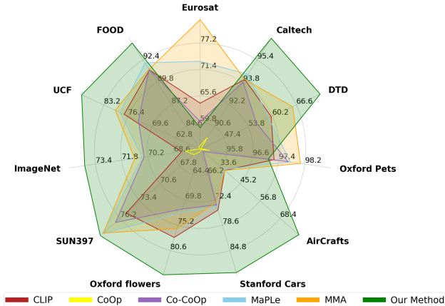
Figure 3. The figure illustrates the superior performance of our model compared to previous state-of-the-art few-shot methods on novel classes. Our approach has demonstrated significant performance gains across multiple challenging datasets, including Stanford Cars, Aircrafts, Oxford Flowers, ImageNet, and Caltech.
