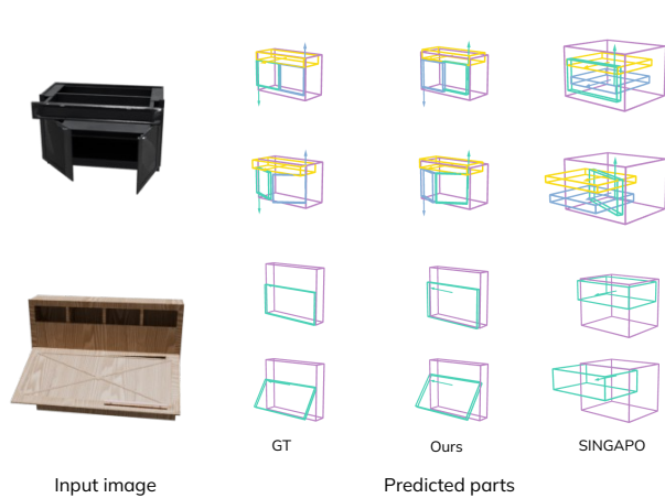
Figure 5. Qualitative comparison with feed-forward baseline of predicted part bounding box and articulation structure.
