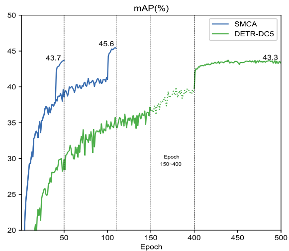
Figure 1. Comparison of DETR-DC5 trained for 500 epochs, and our proposed SMCA trained for 50 epochs and 108 epochs. The convergence speed of the proposed SMCA is faster than DETR.
