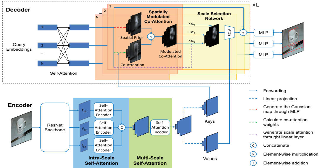
Figure 2. The overall pipeline of Spatially Modulated Co-Attention (SMCA) with intra-scale self-attention, multi-scale self-attention, spatial modulation, and scale-selection attention modules. Each object query performs spatially modulated co-attention and then predicts the target bounding boxes and their object categories. N stands for the number of object queries. L stands for the layers of decoder.
