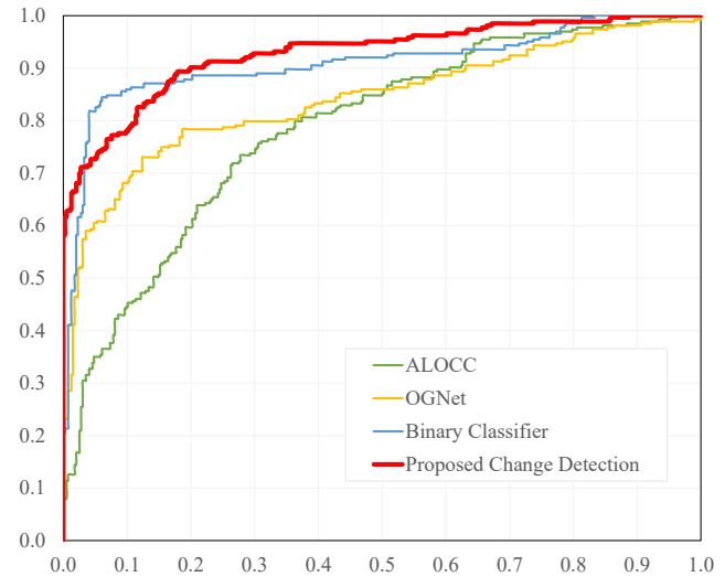
Figure 3. Receiver Operating Characteristic (ROC) curve of our proposed approach and other compared approaches including a convolutional network based binary classifier, OGNet [24], and ALOCC [15].
