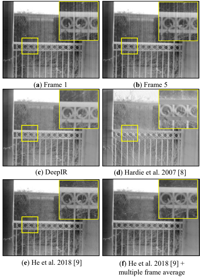
Figure 8: Non-uniformity correction without shutter-based compensation. DeepIR performs comparably to supervised techniques [9] on cameras without built-in shutter-based FFC.
