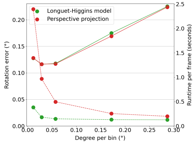
Figure 8. Performance on BUSS as a function of bin size. Our method’s accuracy (continuous line) and run time (dashed line) with perspective projection and Longuet-Higgins. The methods have similar accuracy but Longuet-Higgins is much faster.
