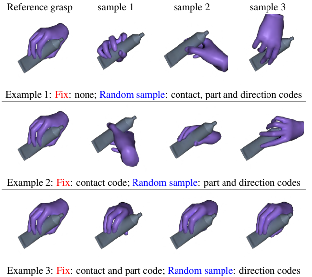
Figure 8: Visualizing grasp diversity by selectively fixing contact code, part code, and direction code.. In the top row, grasps use random contact, part, and direction codes. In the middle row, contact is fixed, only part and direction vary. In the bottom row, contact and part are fixed, only direction changes.
