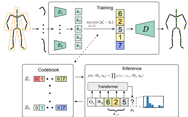
Figure 3. Part VQ-VAE. Part VQ-VAE first splits the skeleton into multiple parts and learns the codebooks separately. The composition of different parts is subsequently modeled with the autoregressive prediction model.
